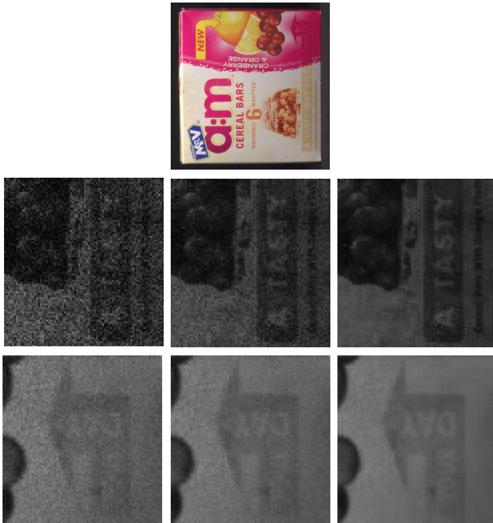
Figure 2. Results of multispectral image denoising of the test image number 12 from the database [8]. From top to bottom: MS image (sRGB values rendered under a neutral daylight, D65), fragment of the 1st spectral component, different fragment of 31st spectral component. From left to right: noisy image, denoised by multispectral modification of CBM3D and denoised by proposed algorithm.
