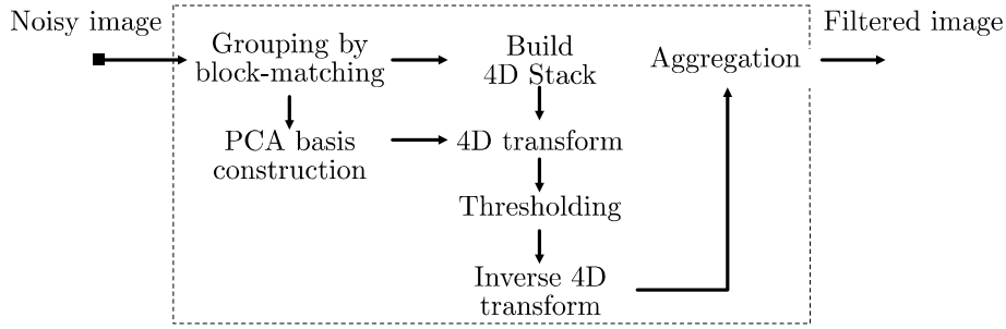
Figure 1. Flowchart of the proposed MSPCA-BM3D algorithm.
