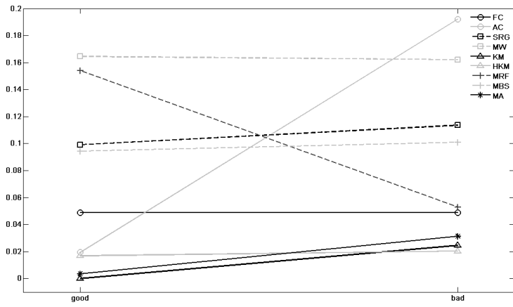
Figure 5. The interaction plot shows how the probability of error for each algorithm changes while quality of analyzed images degrades.
