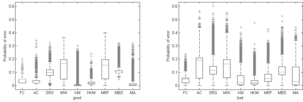
Figure 3. Boxplots illustrating the distribution of the probability of error measured for both good and low quality images.
