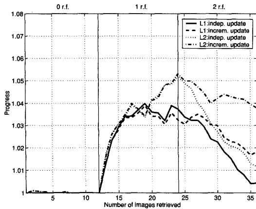
Figure 2: Average progress for the first two iterations.
