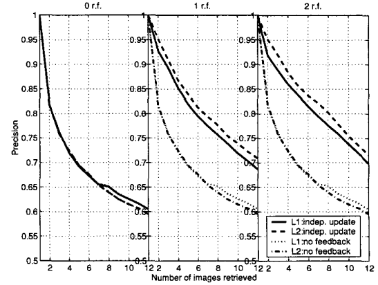
Figure 1: Average precision for the first two iterations.
