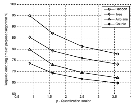
Fig.2 Required encoding time of the proposed detection algorithm compared to the baseline JPEG encoder
