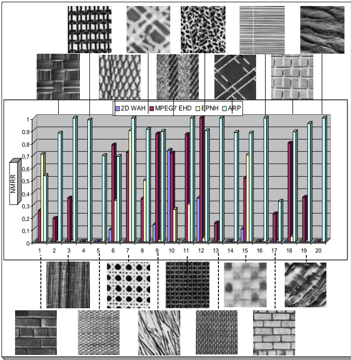
Figure 3: ANMRR plots of 4 methods for 20 queries over Texture database.
