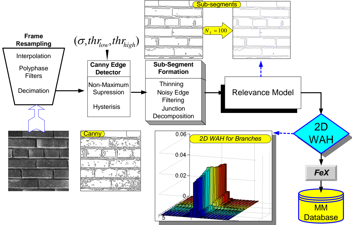
Figure 1: Overview of the 2D WAH as a texture descriptor.
