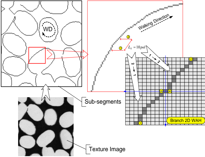
Figure 2: Localization of a branch LoS into 2D WAH.
