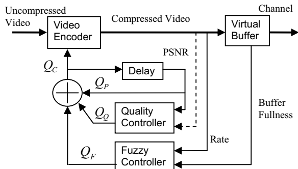
Figure 1. Block diagram of the fuzzy video rate controller.
