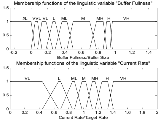
Figure 2. Membership function of the linguistic variables
