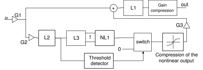
Fig. 1. Proposed model topology
