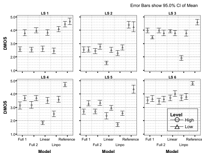
Fig. 3. Degradation mean opinion score (DMOS) values with 95% confidence intervals for all subjects averaged across PROGRAM
