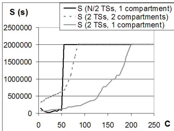
FIG. 14: Average S vs. average C for a single TS. 100 experiments per data point. The system goes through a phase transition from oscillating to stable. For comparison, the two previous cases are plotted (2 TSs in 1 compartment and 2 TSs in 2 compartments)
