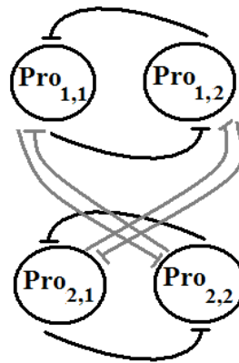
FIG. 1: Two coupled TSs in a single compartment.
