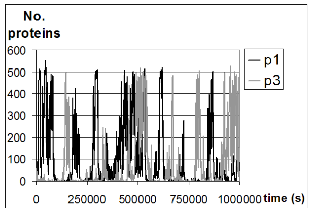
FIG. 7: Two TSs uncoupled ( k_c = 0 s^{-1} ). Time series of proteins p_1 and p_3 (corresponding to genes “1” of each of the toggles). The oscillations of the two TSs are not correlated.
