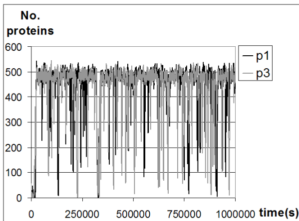
FIG. 9: Two coupled TSs: k_c = 0.1s^{-1} . Time series of p_1 and p_3 . The two TSs oscillate synchronously, but at a lower frequency than in Fig 8.
