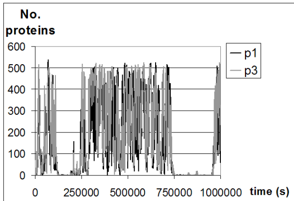
FIG. 9: Two coupled TSs: k_c = 0.1s^{-1} . Time series of p_1 and p_3 . The two TSs oscillate synchronously, but at a lower frequency than in Fig 8.
