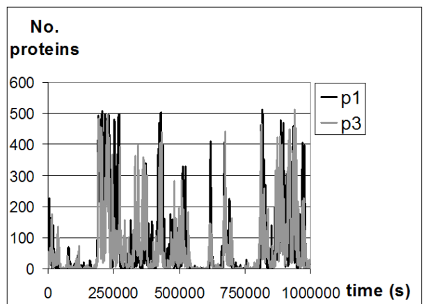
FIG. 7: Two TSs uncoupled ( k_c = 0 s^{-1} ). Time series of proteins p_1 and p_3 (corresponding to genes “1” of each of the toggles). The oscillations of the two TSs are not correlated.
