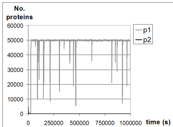
FIG. 4: Time series of a TS with 100 s delays on the proteins release and no cooperative binding. As in case A, after a transient, the system remains stable and the number of proteins of the repressed gene ( p_2 ) never goes beyond 20, except during the initial transient (unlike in case A), due to the delay on the proteins release.
